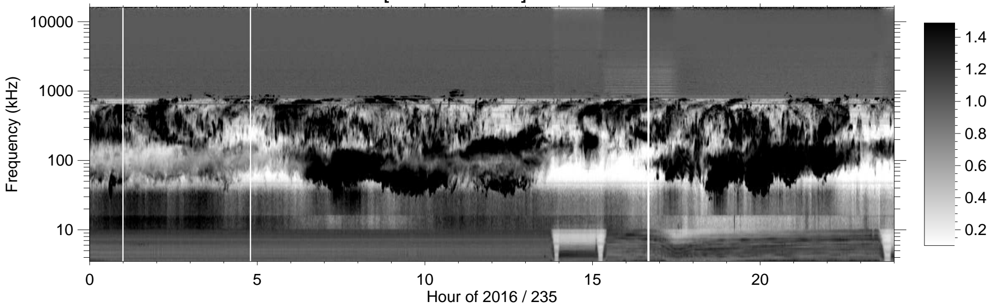
RPWS [ABCH1H2/Ex] (-B) 2016/08/22
