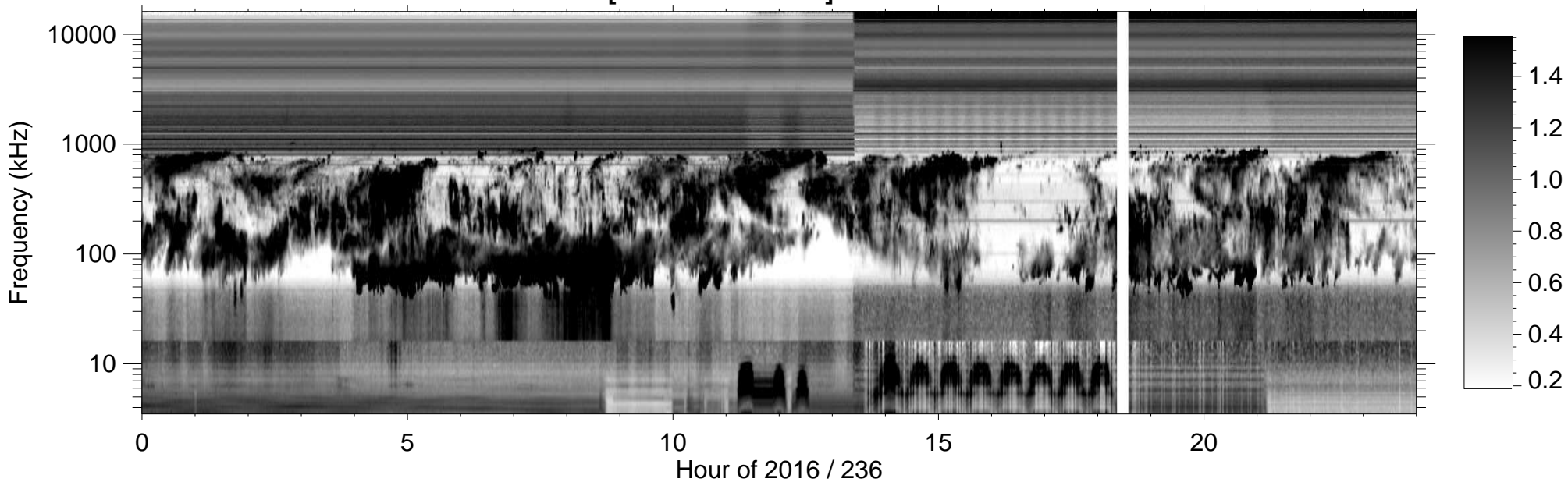
RPWS [ABCH1H2/Ex] (-B) 2016/08/23
