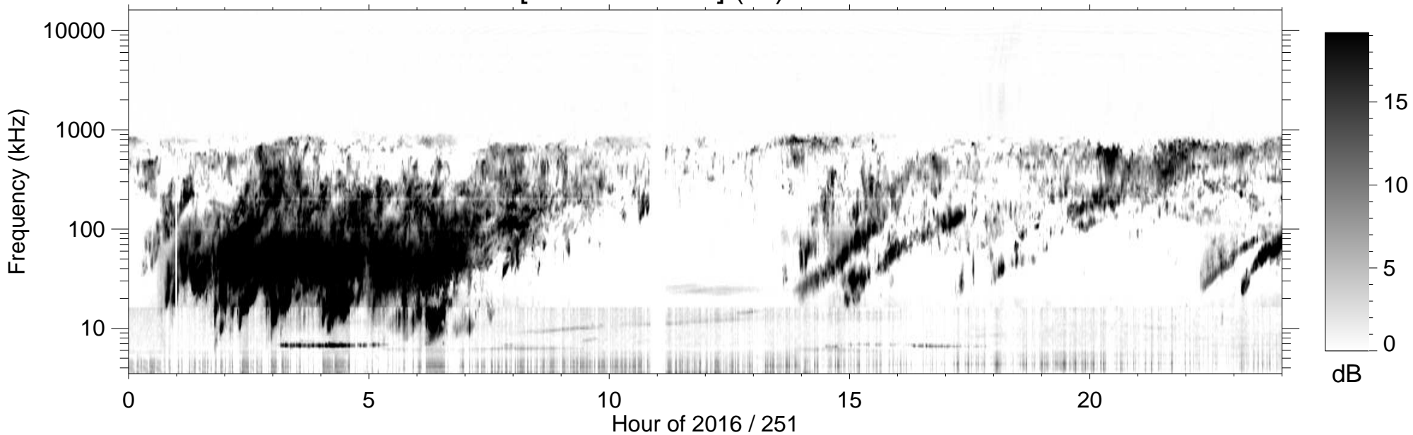
RPWS [ABCH1H2/Ex] (-B) 2016/09/07
