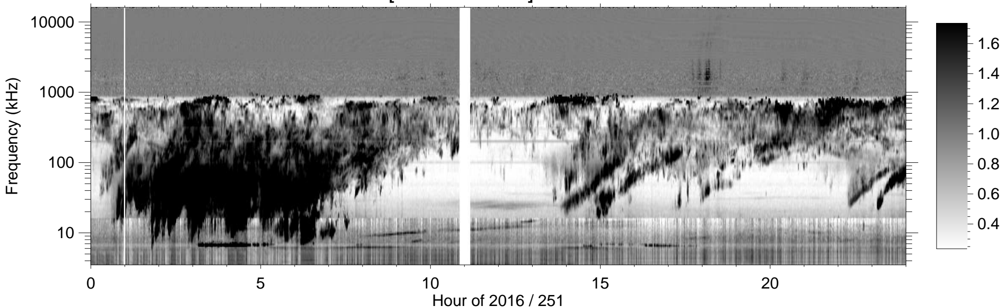
RPWS [ABCH1H2/Ex] (-B) 2016/09/07
