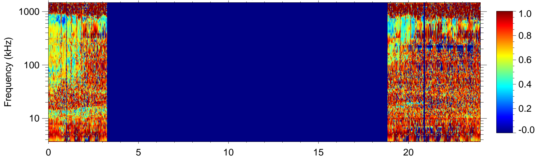
Total polarization
