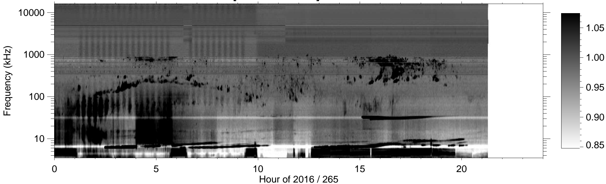
RPWS [ABCH1H2/Ex] (-B) 2016/09/21
