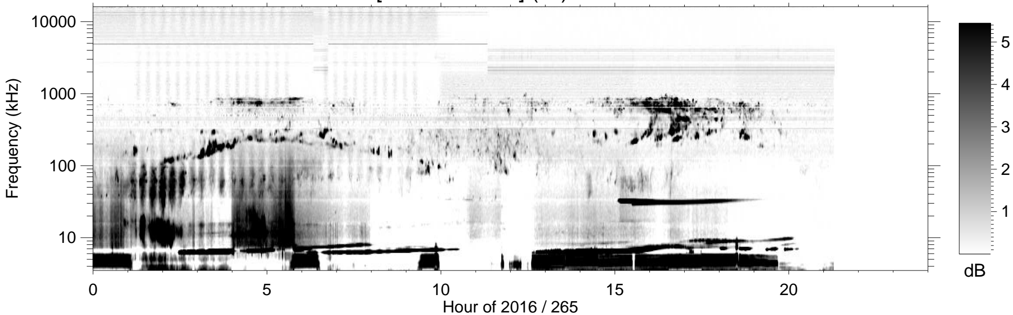
RPWS [ABCH1H2/Ex] (-B) 2016/09/21
