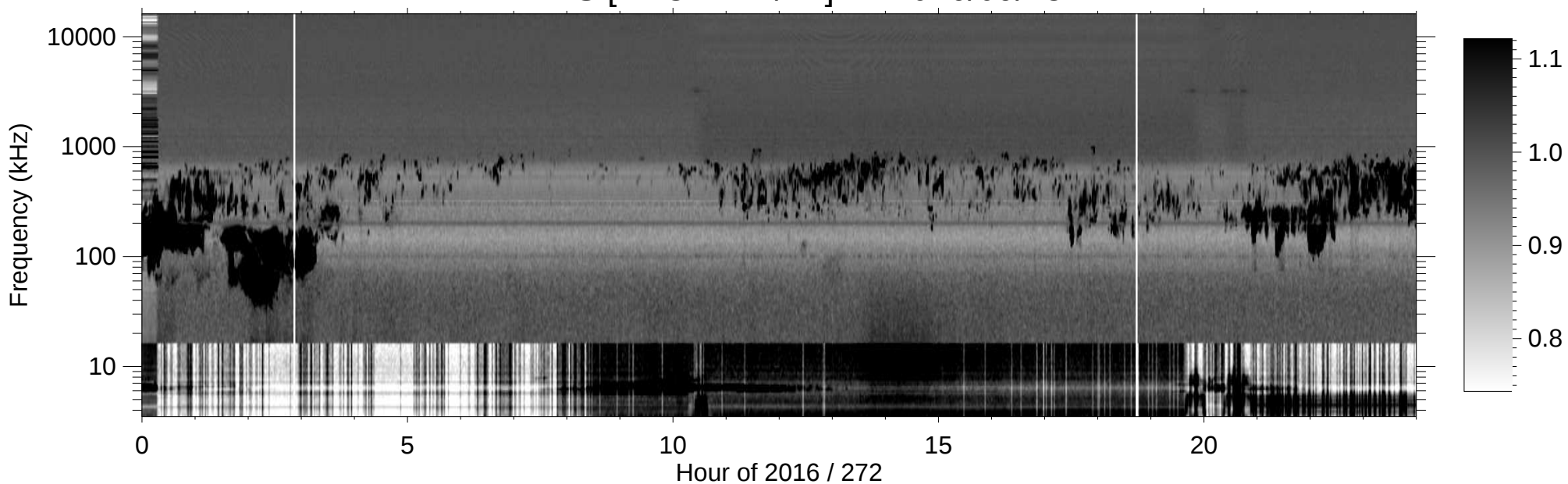
RPWS [ABCH1H2/Ex] (-B) 2016/09/28
