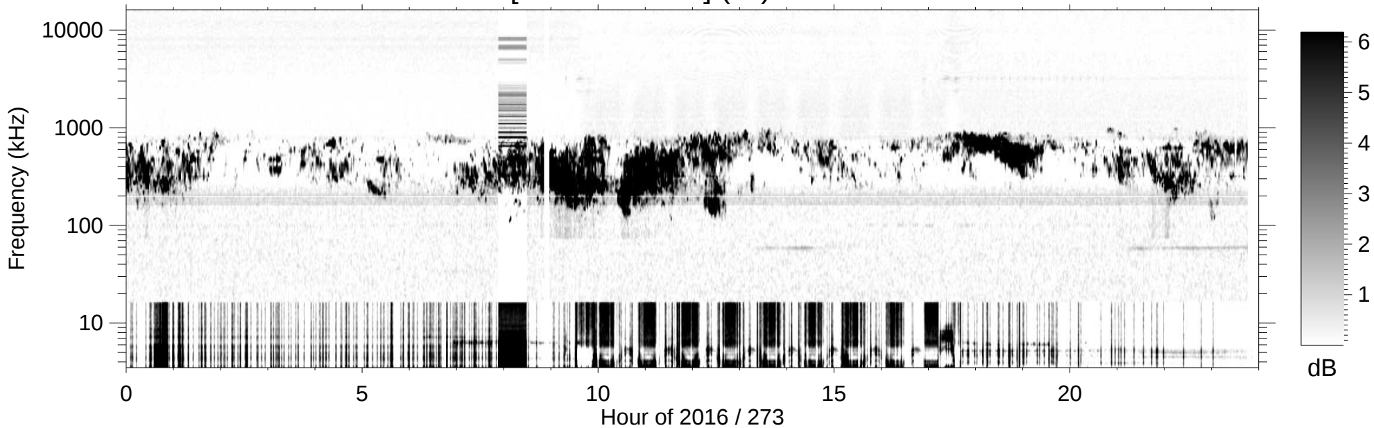
RPWS [ABCH1H2/Ex] (-B) 2016/09/29
