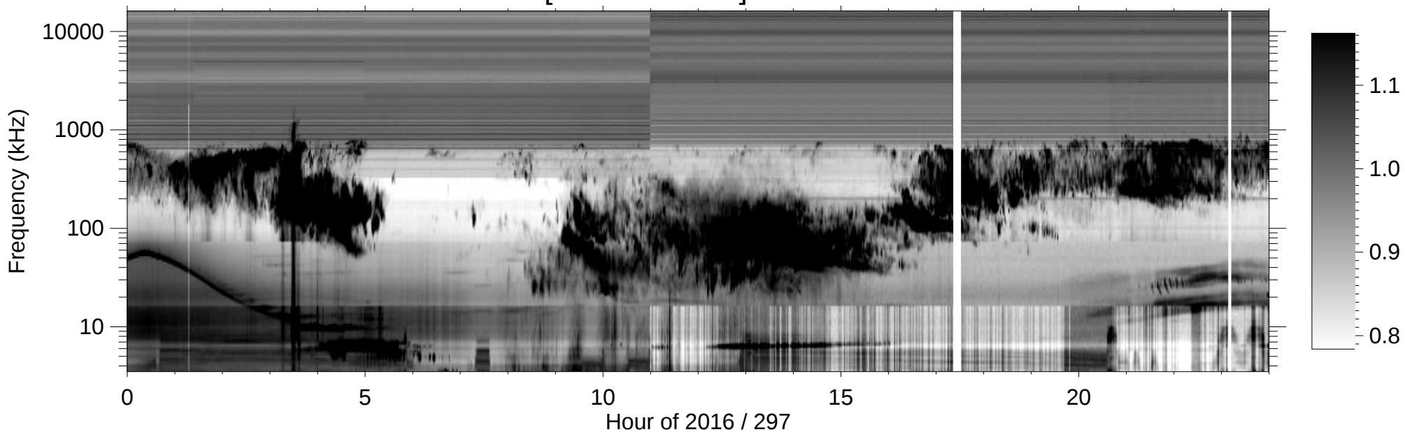
RPWS [ABCH1H2/Ex] (-B) 2016/10/23
