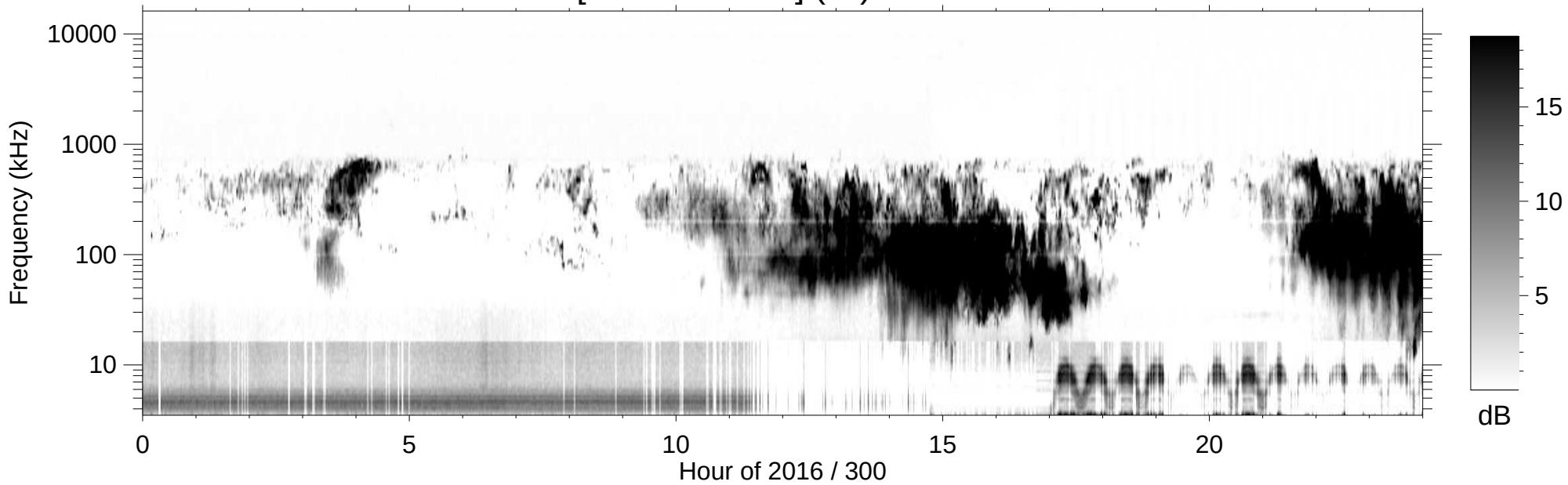
RPWS [ABCH1H2/Ex] (-B) 2016/10/26
