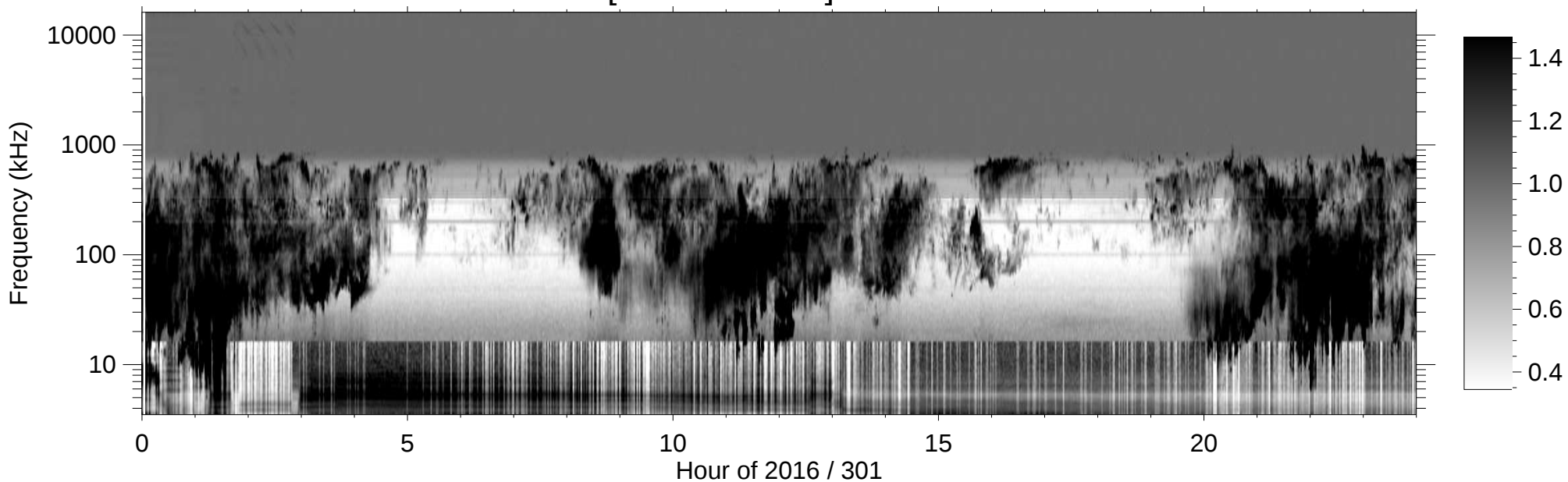
RPWS [ABCH1H2/Ex] (-B) 2016/10/27
