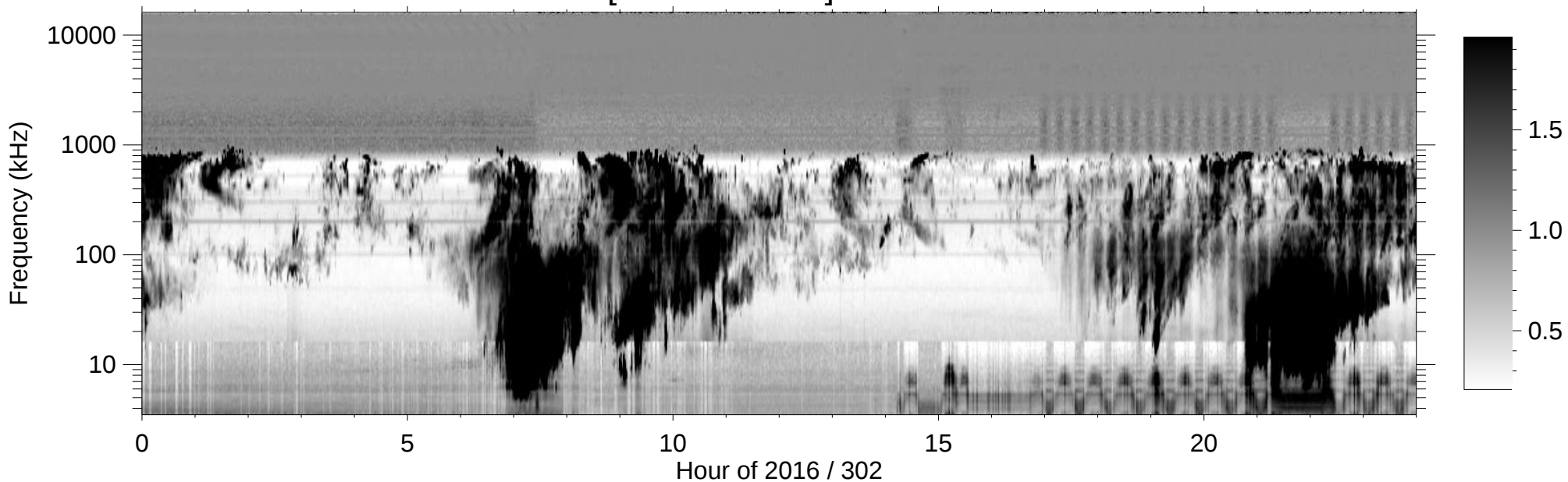
RPWS [ABCH1H2/Ex] (-B) 2016/10/28
