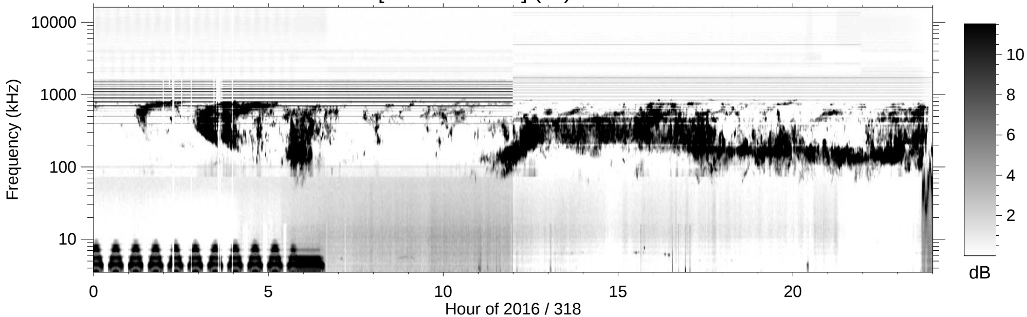
RPWS [ABCH1H2/Ex] (-B) 2016/11/13
