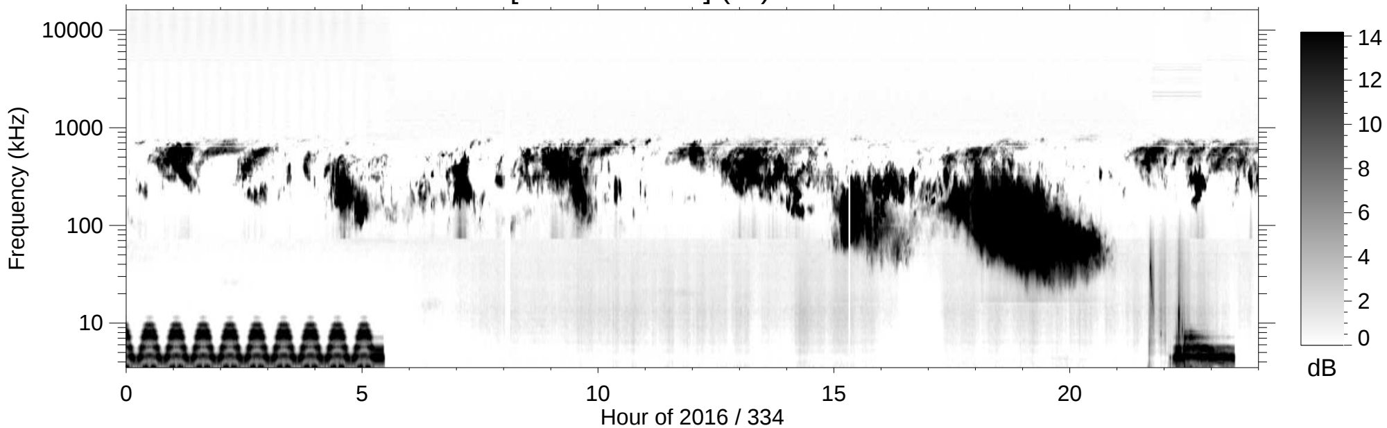
RPWS [ABCH1H2/Ex] (-B) 2016/11/29
