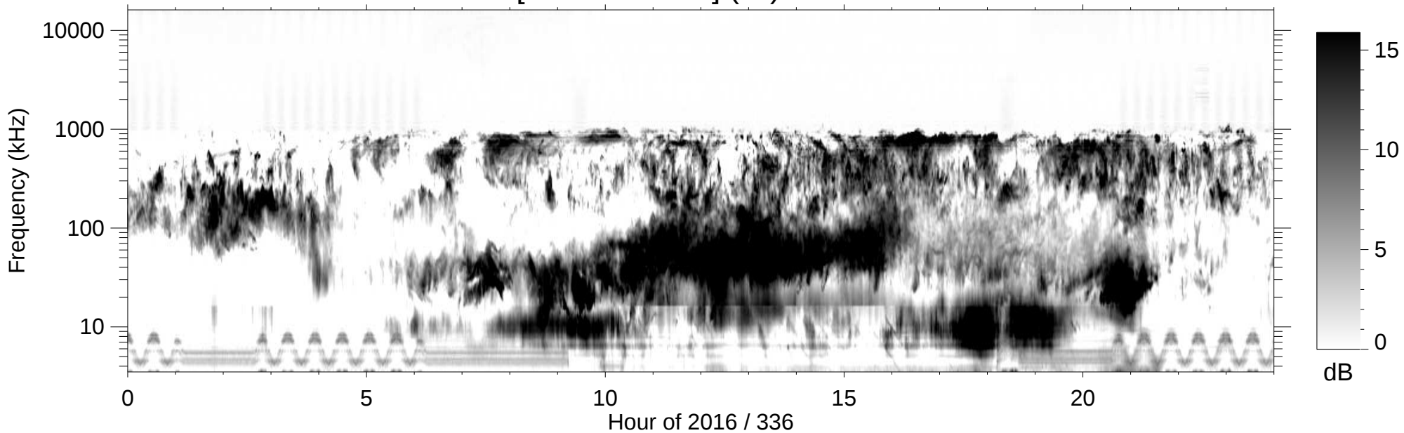
RPWS [ABCH1H2/Ex] (-B) 2016/12/01
