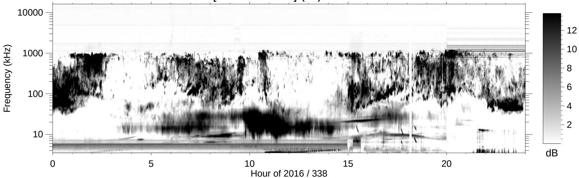
RPWS [ABCH1H2/Ex] (-B) 2016/12/03
