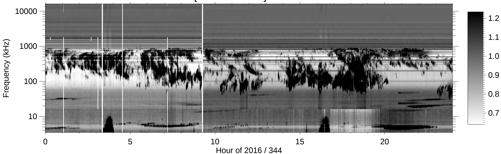
RPWS [ABCH1H2/Ex] (-B) 2016/12/09
