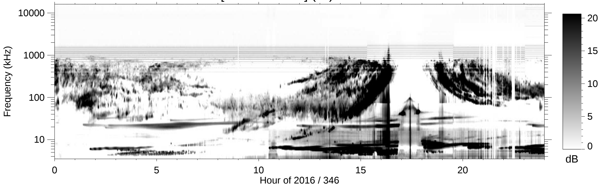
RPWS [ABCH1H2/Ex] (-B) 2016/12/11
