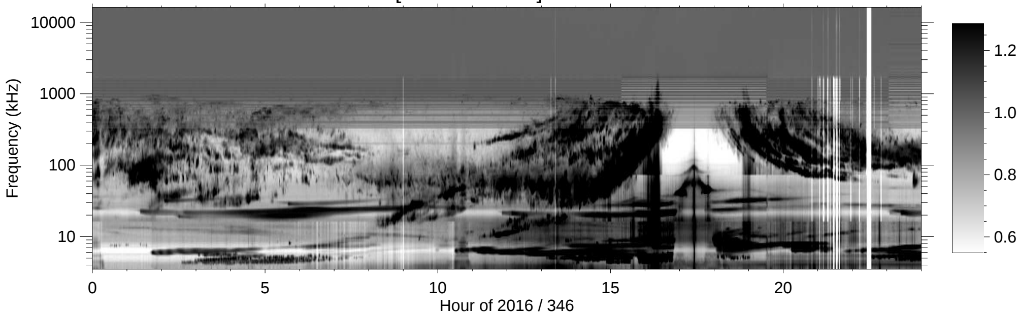
RPWS [ABCH1H2/Ex] (-B) 2016/12/11
