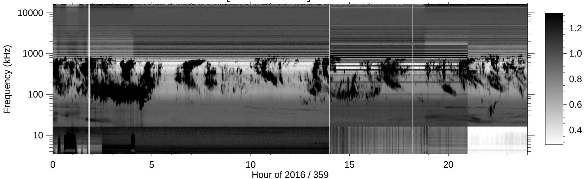
RPWS [ABCH1H2/Ex] (-B) 2016/12/24
