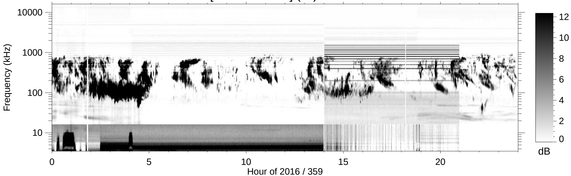
RPWS [ABCH1H2/Ex] (-B) 2016/12/24
