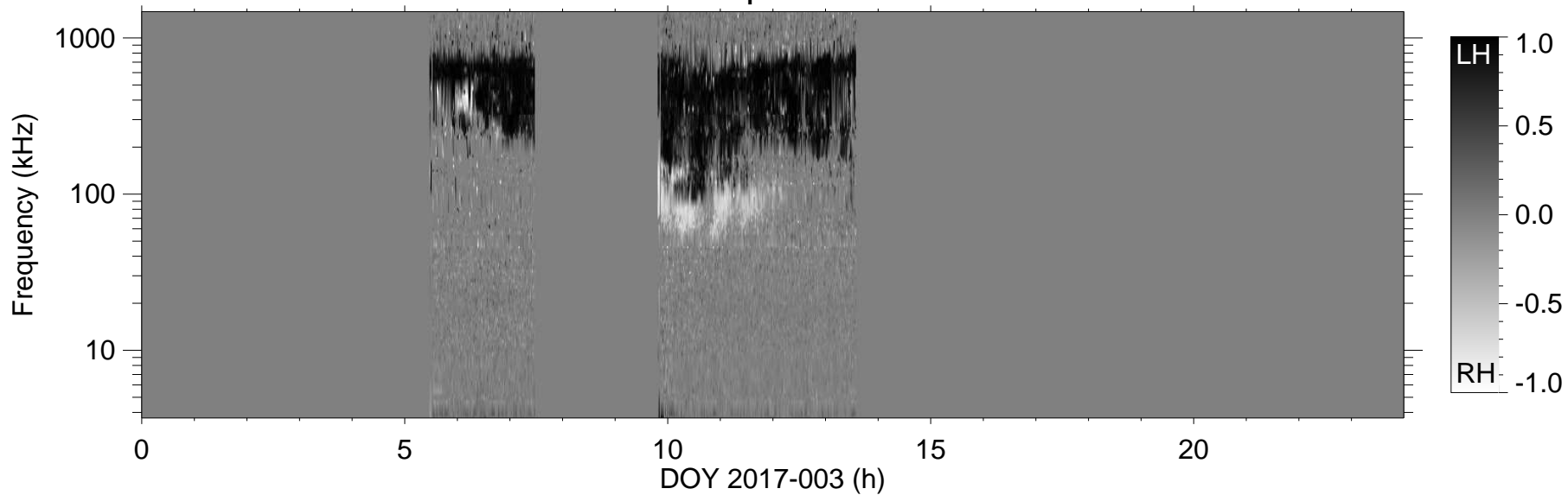
Circular polarization
