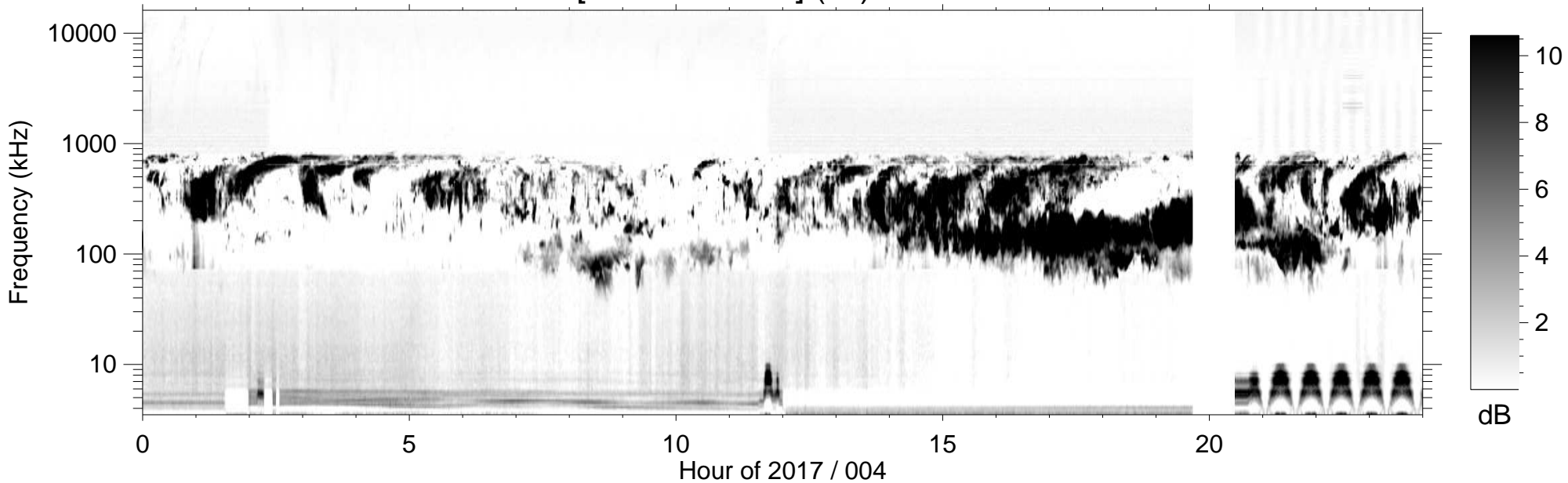
RPWS [ABCH1H2/Ex] (-B) 2017/01/04
