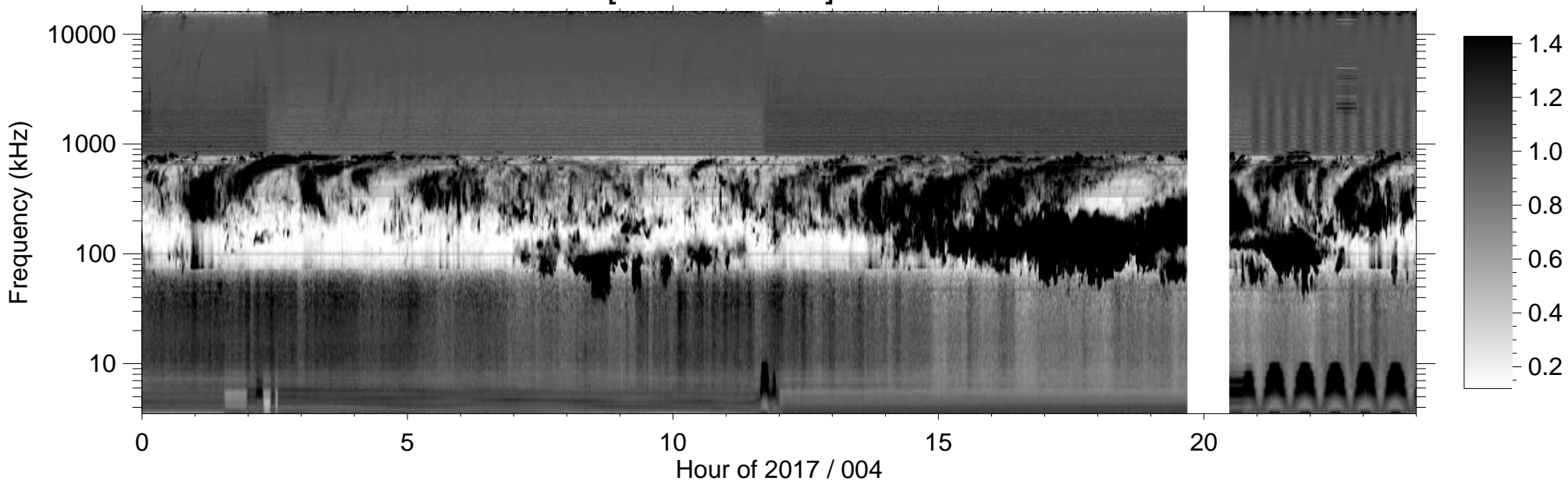
RPWS [ABCH1H2/Ex] (-B) 2017/01/04
