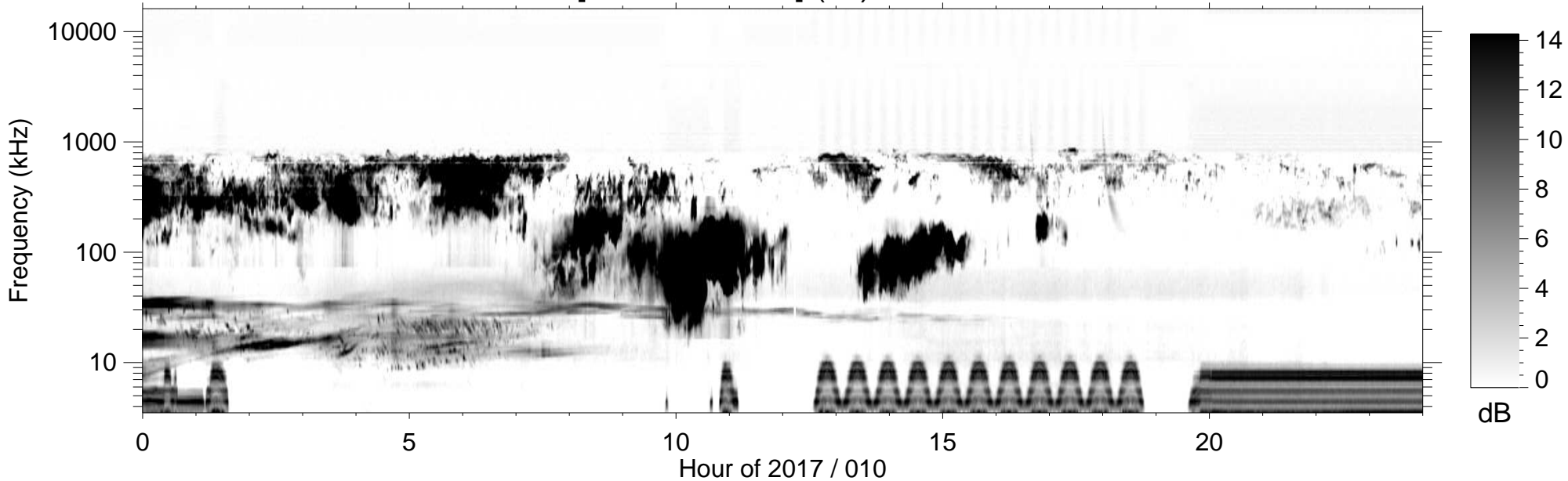
RPWS [ABCH1H2/Ex] (-B) 2017/01/10
