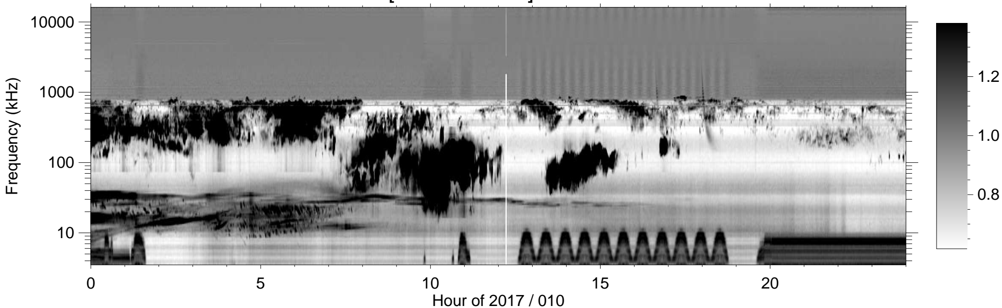
RPWS [ABCH1H2/Ex] (-B) 2017/01/10
