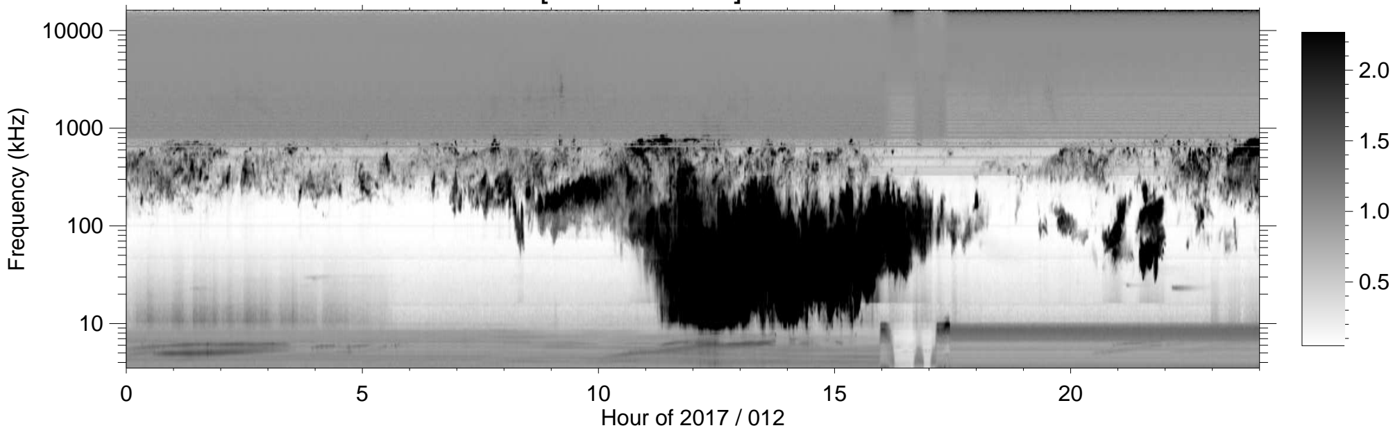
RPWS [ABCH1H2/Ex] (-B) 2017/01/12
