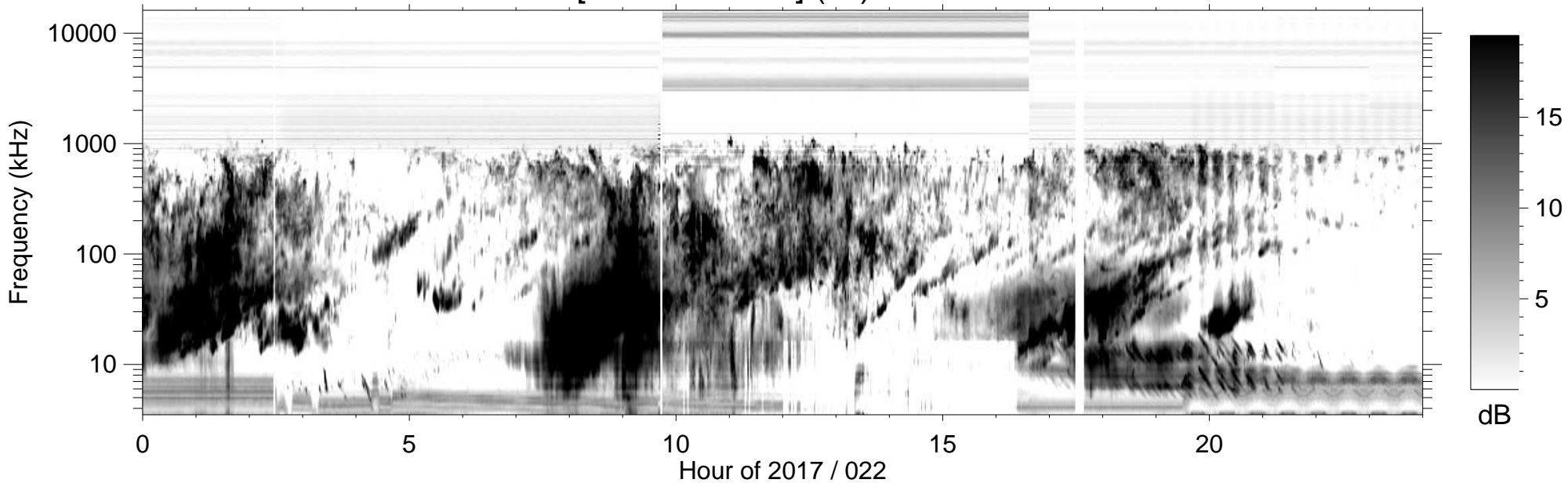
RPWS [ABCH1H2/Ex] (-B) 2017/01/22
