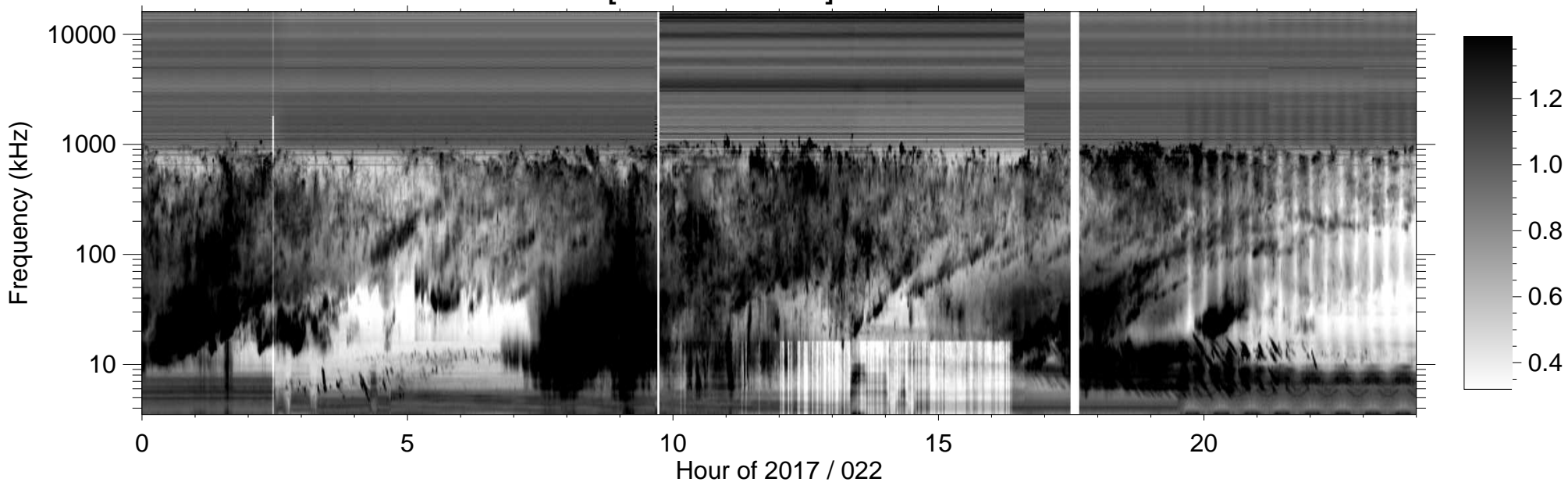
RPWS [ABCH1H2/Ex] (-B) 2017/01/22
