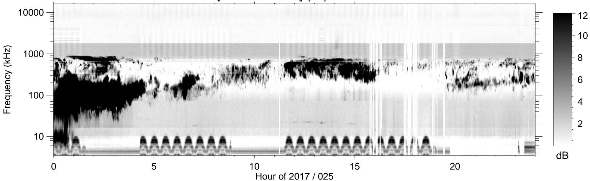
RPWS [ABCH1H2/Ex] (-B) 2017/01/25
