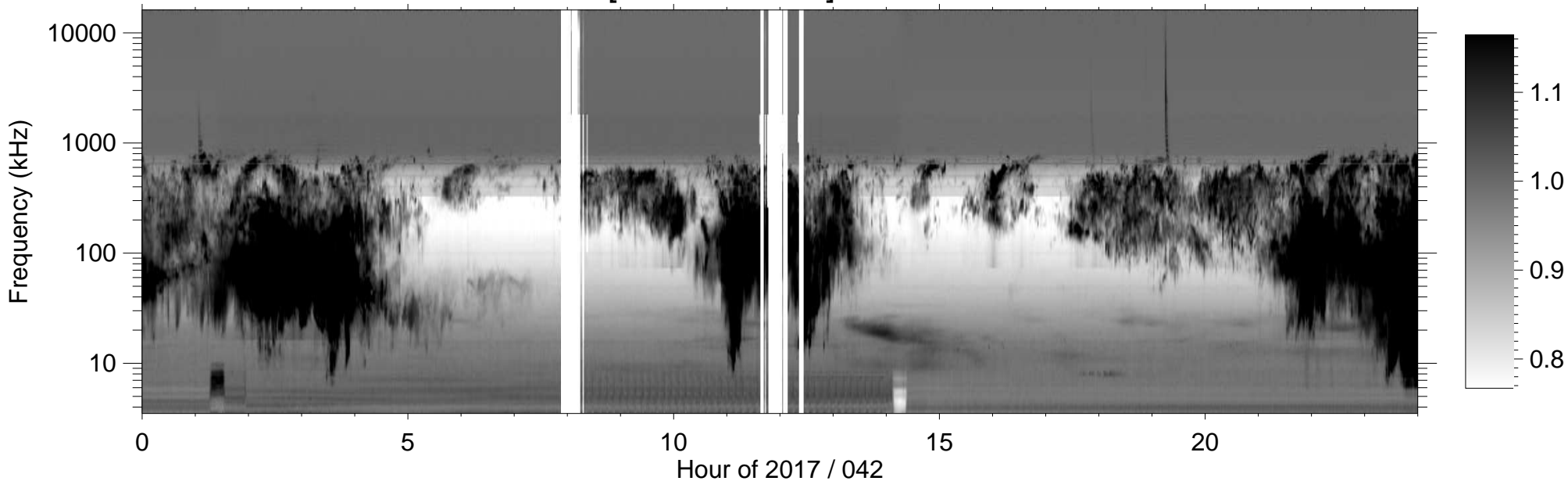
RPWS [ABCH1H2/Ex] (-B) 2017/02/11
