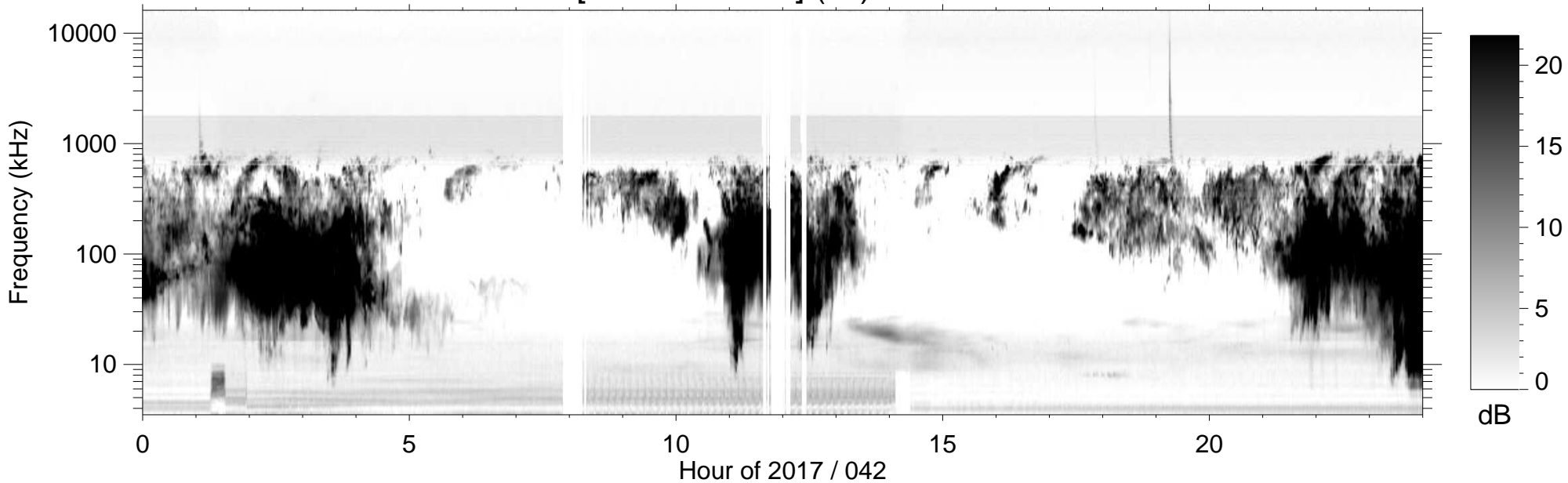
RPWS [ABCH1H2/Ex] (-B) 2017/02/11
