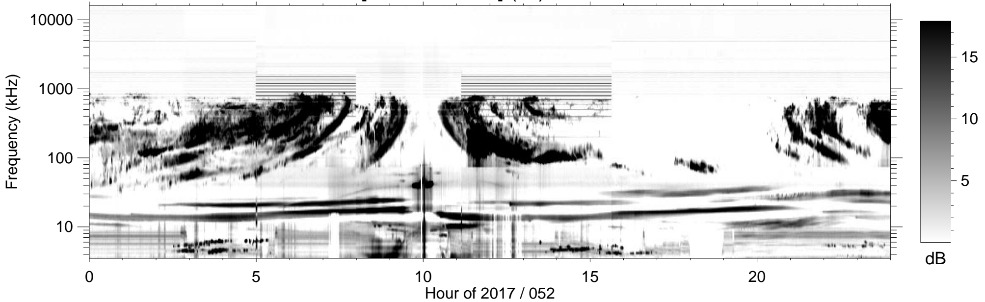
RPWS [ABCH1H2/Ex] (-B) 2017/02/21
