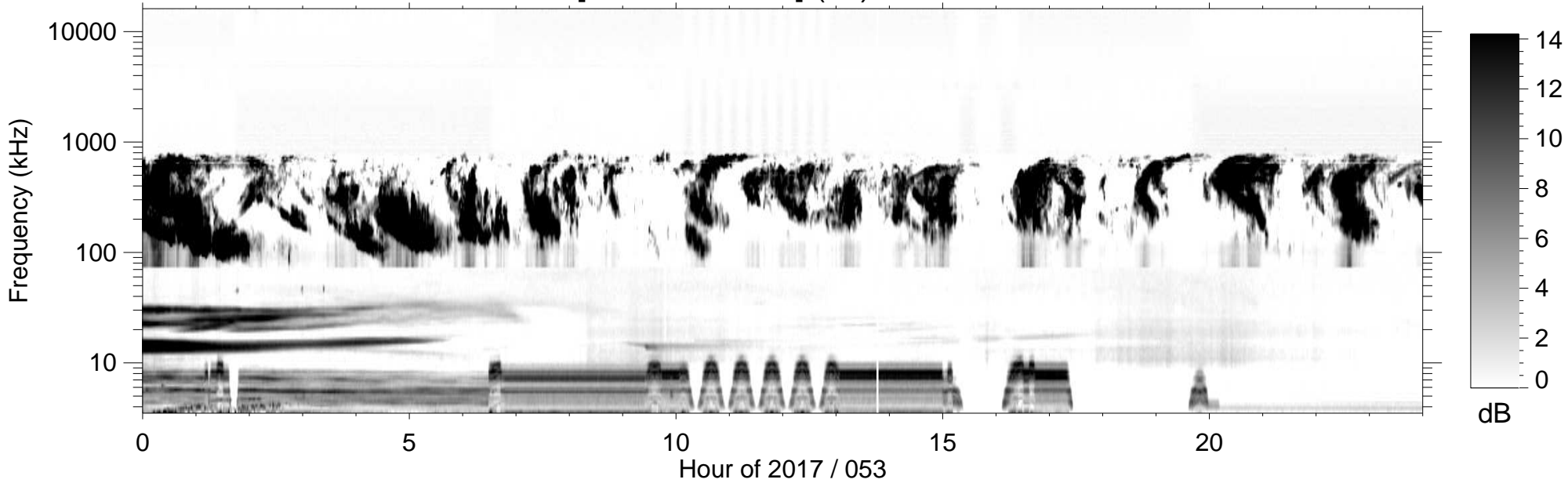
RPWS [ABCH1H2/Ex] (-B) 2017/02/22
