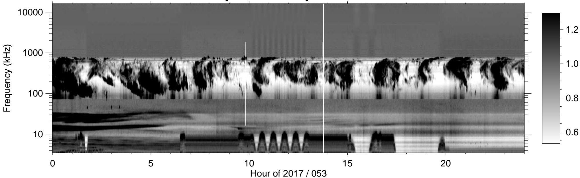
RPWS [ABCH1H2/Ex] (-B) 2017/02/22
