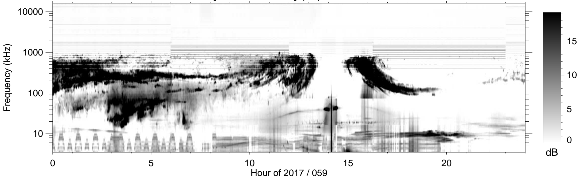
RPWS [ABCH1H2/Ex] (-B) 2017/02/28
