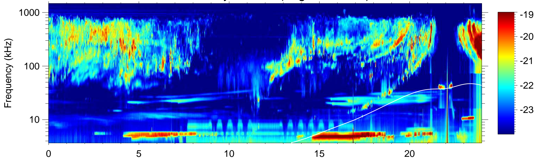
Circular polarization
