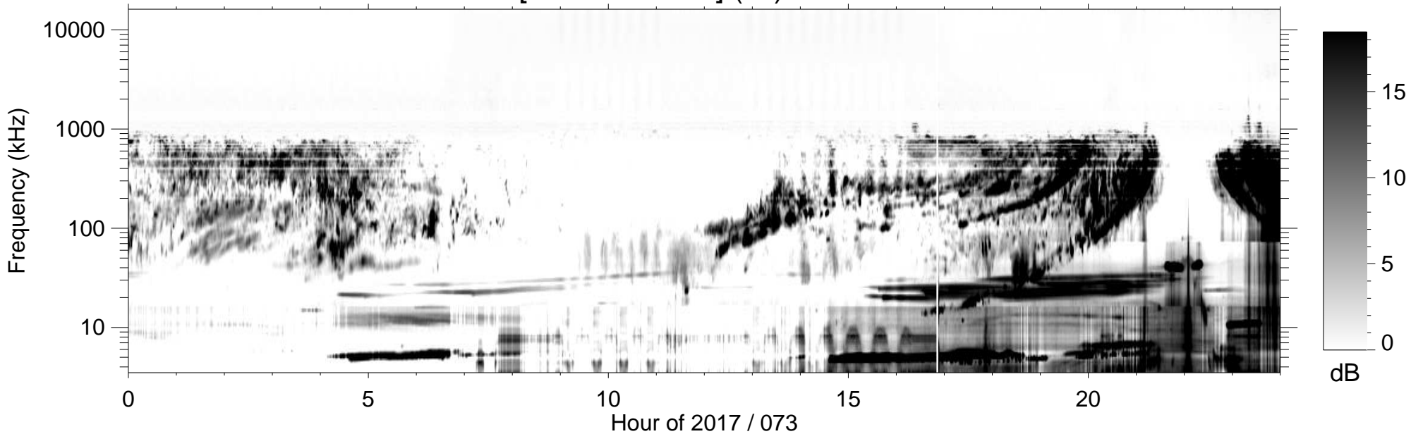
RPWS [ABCH1H2/Ex] (-B) 2017/03/14
