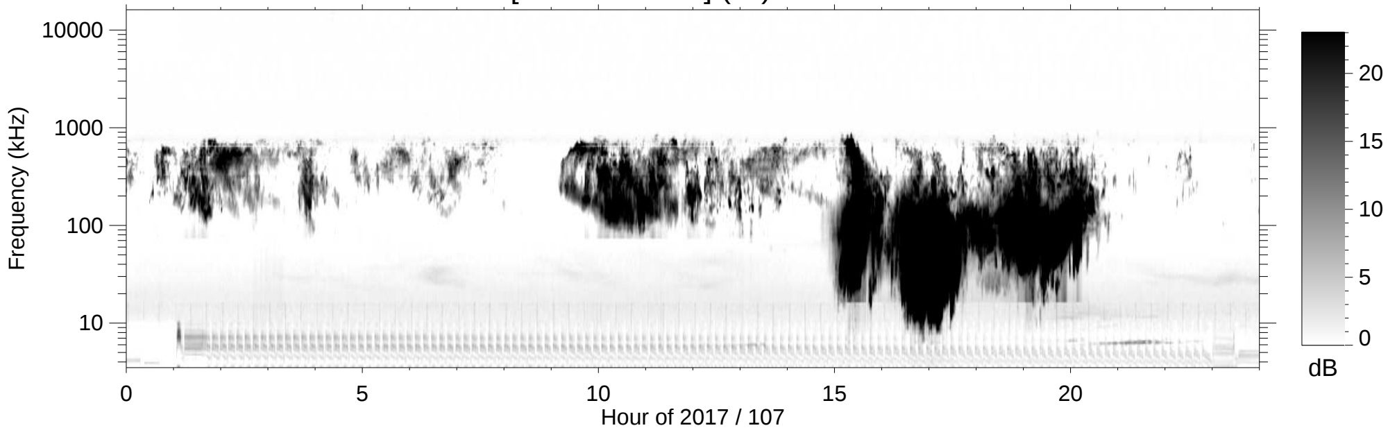
RPWS [ABCH1H2/Ex] (-B) 2017/04/17
