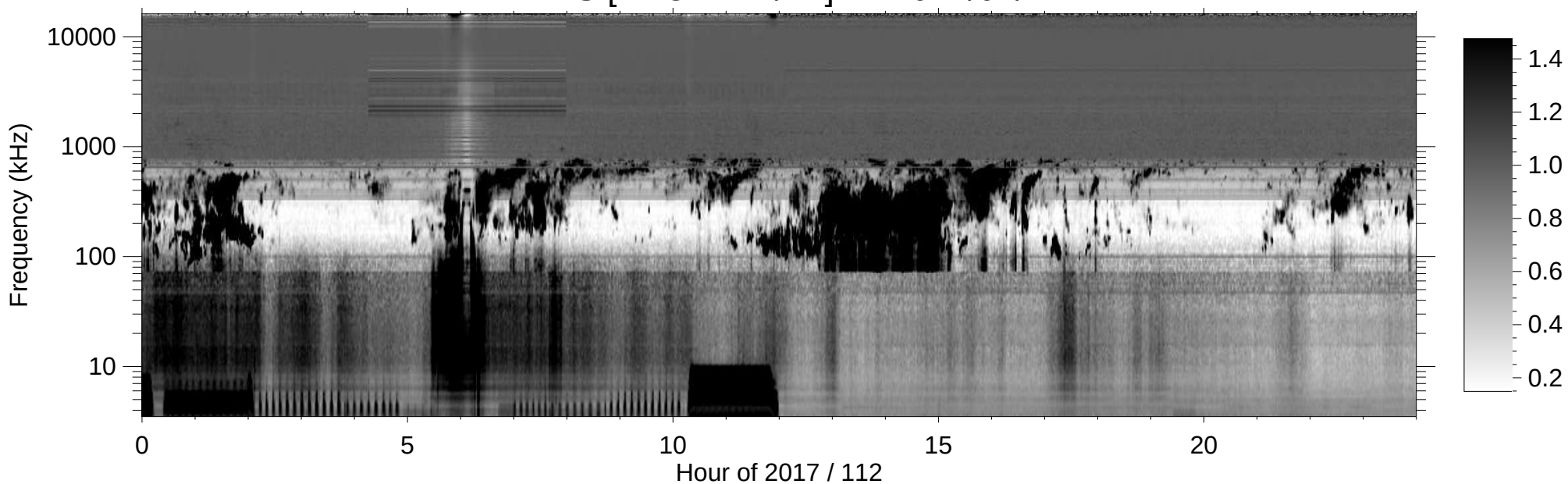
RPWS [ABCH1H2/Ex] (-B) 2017/04/22
