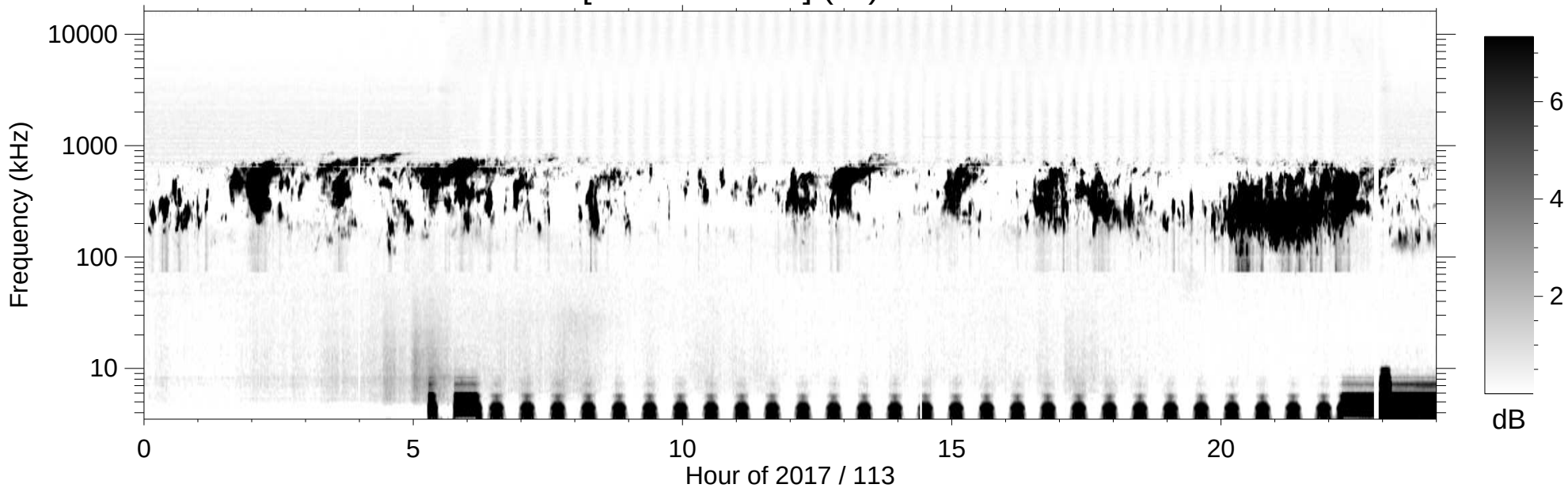
RPWS [ABCH1H2/Ex] (-B) 2017/04/23
