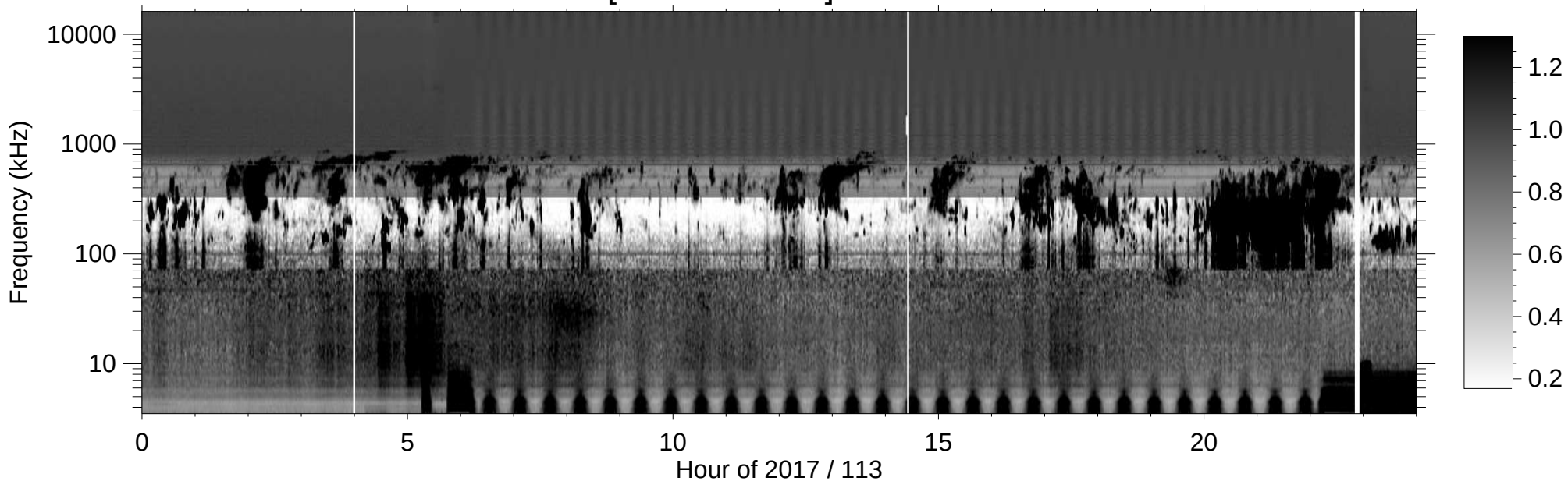
RPWS [ABCH1H2/Ex] (-B) 2017/04/23
