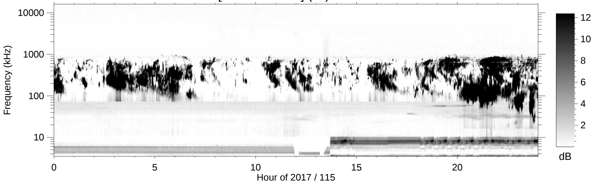
RPWS [ABCH1H2/Ex] (-B) 2017/04/25
