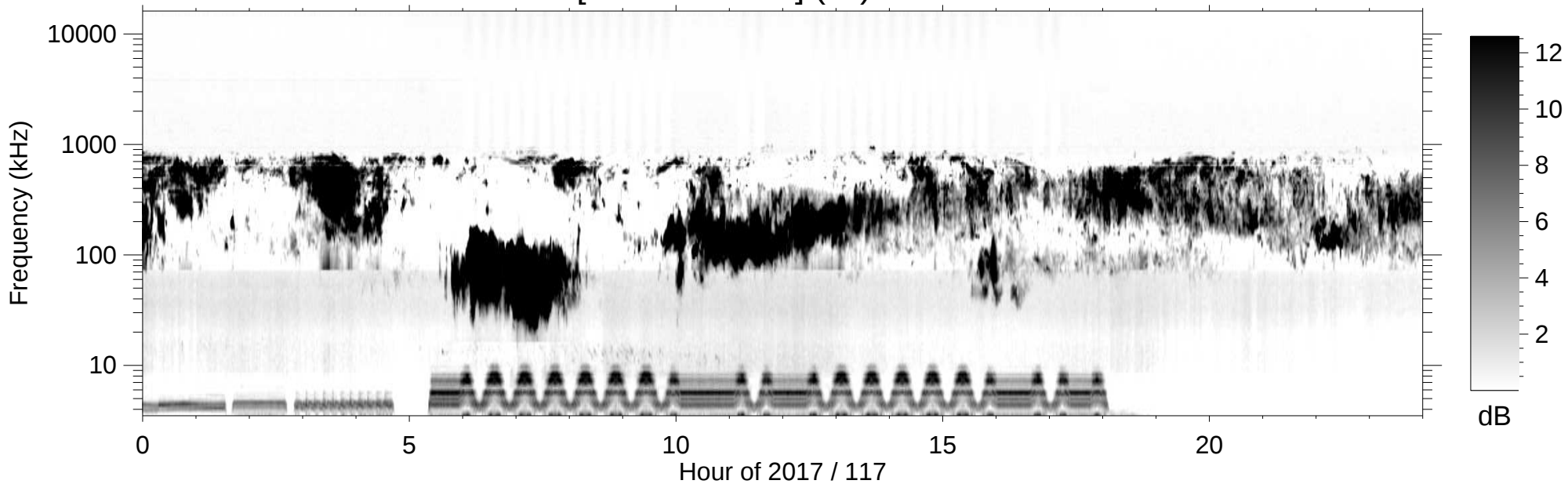
RPWS [ABCH1H2/Ex] (-B) 2017/04/27
