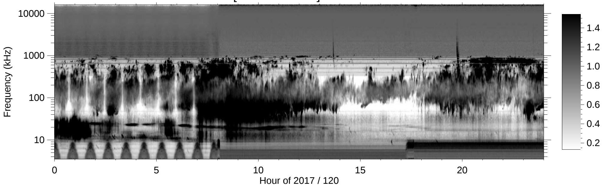
RPWS [ABCH1H2/Ex] (-B) 2017/04/30
