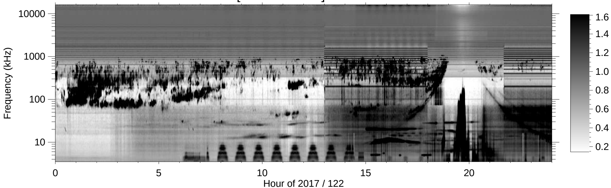
RPWS [ABCH1H2/Ex] (-B) 2017/05/02
