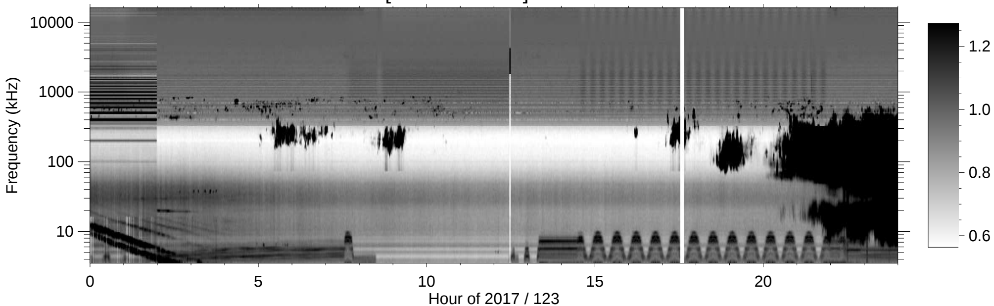
RPWS [ABCH1H2/Ex] (-B) 2017/05/03
