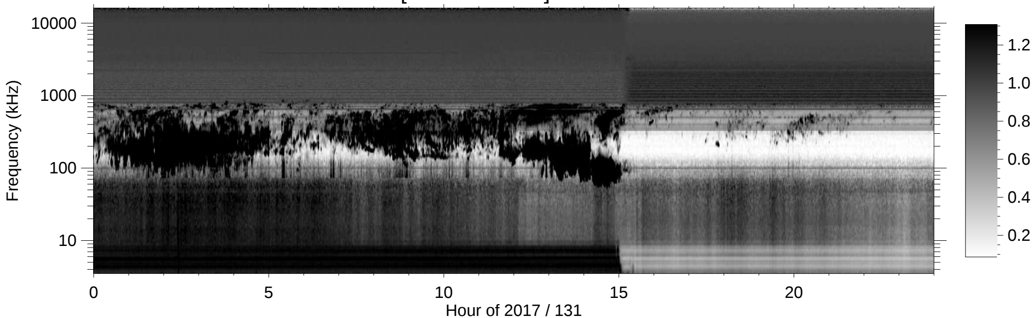
RPWS [ABCH1H2/Ex] (-B) 2017/05/11
