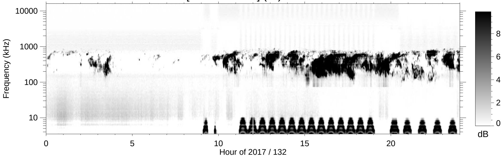
RPWS [ABCH1H2/Ex] (-B) 2017/05/12
