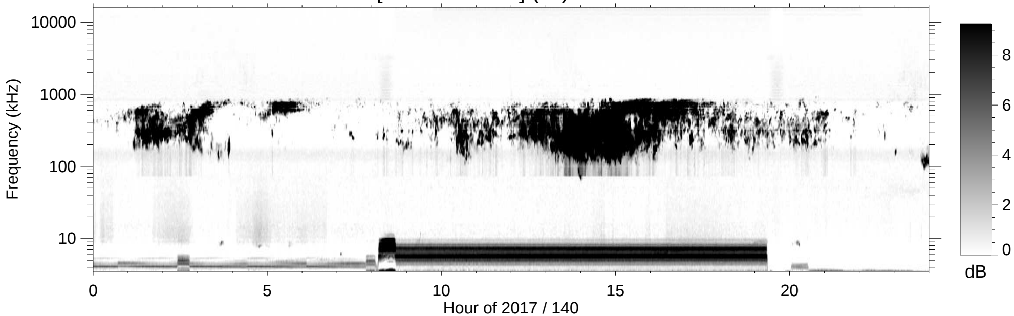
RPWS [ABCH1H2/Ex] (-B) 2017/05/20
