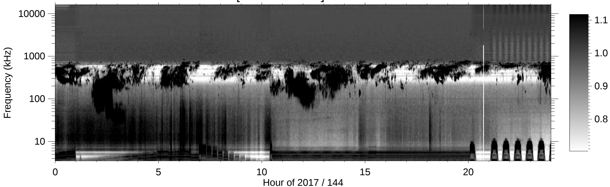
RPWS [ABCH1H2/Ex] (-B) 2017/05/24
