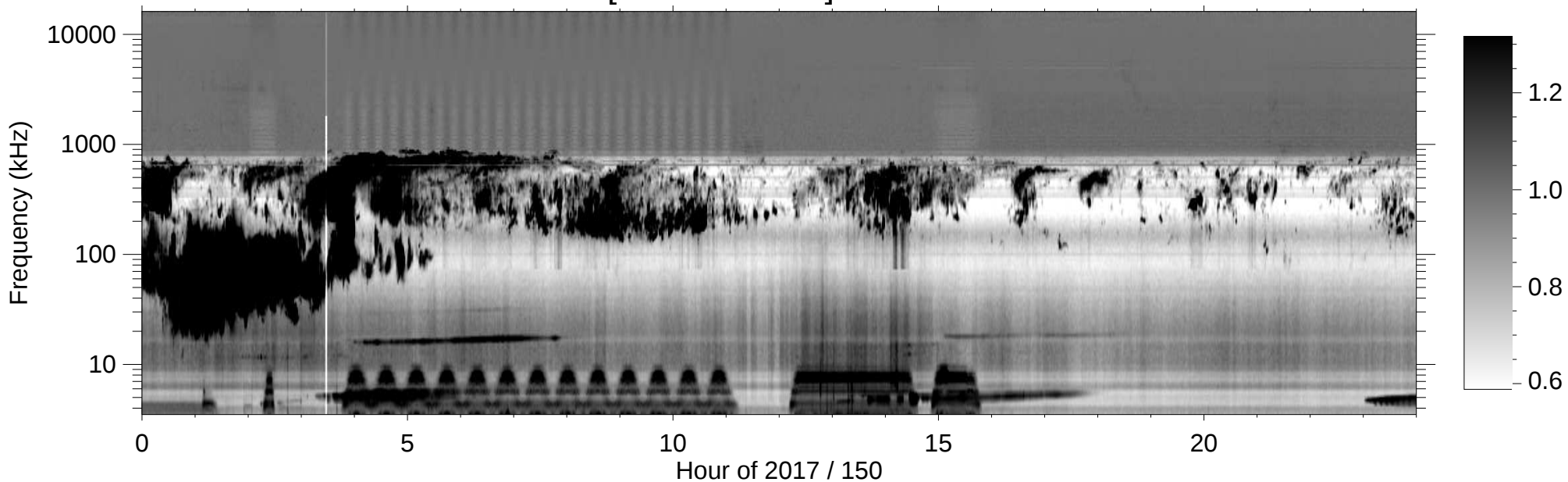
RPWS [ABCH1H2/Ex] (-B) 2017/05/30
