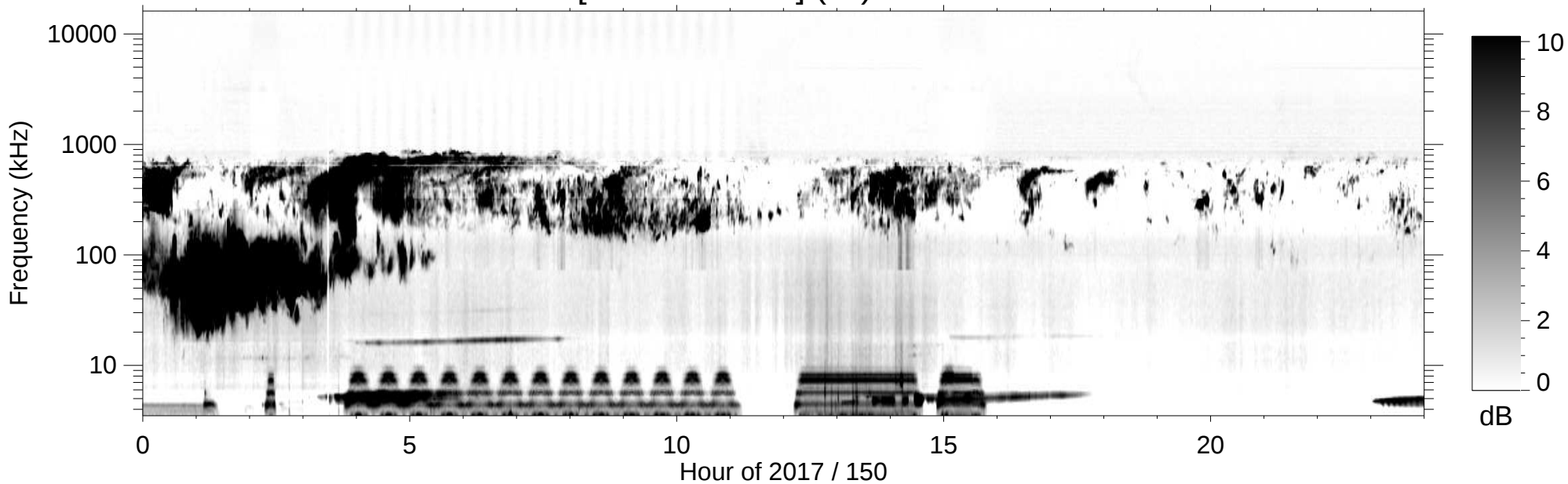
RPWS [ABCH1H2/Ex] (-B) 2017/05/30
