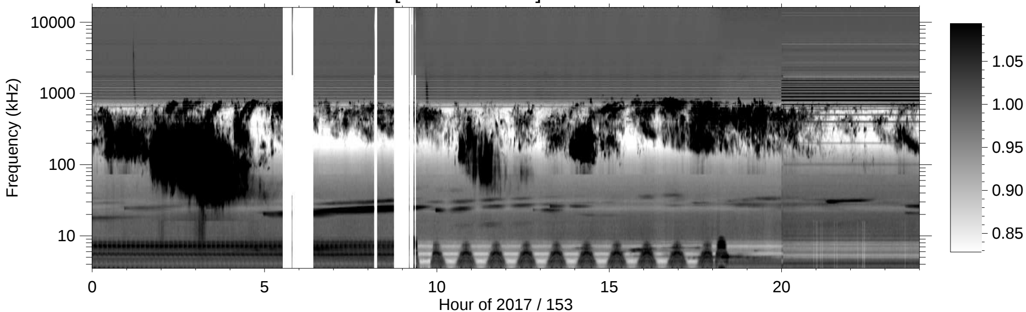
RPWS [ABCH1H2/Ex] (-B) 2017/06/02
