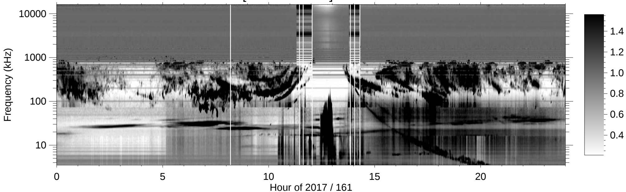
RPWS [ABCH1H2/Ex] (-B) 2017/06/10
