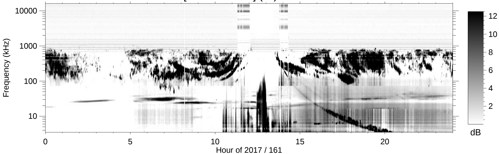
RPWS [ABCH1H2/Ex] (-B) 2017/06/10
