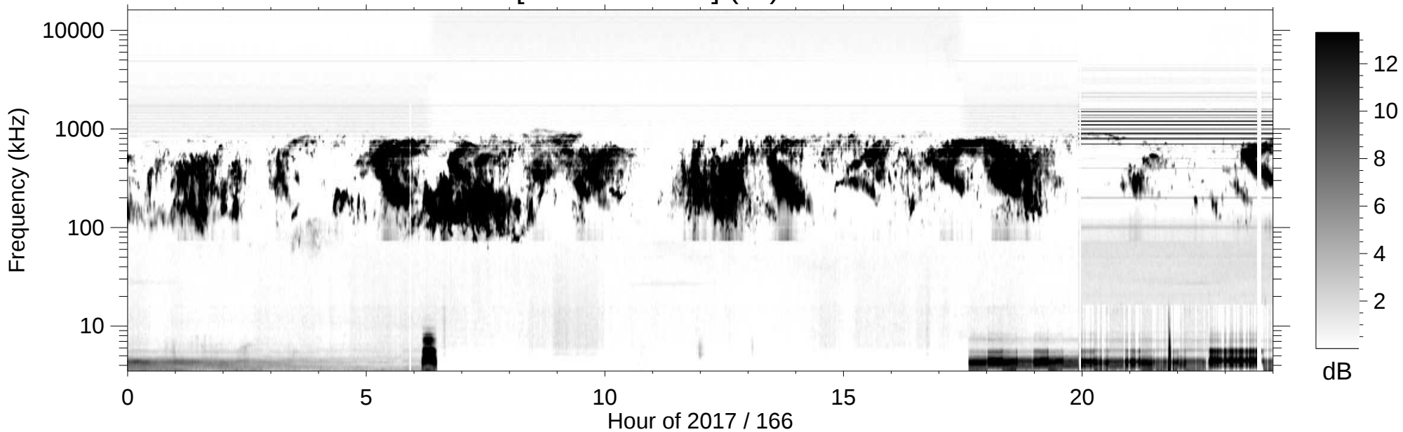
RPWS [ABCH1H2/Ex] (-B) 2017/06/15
