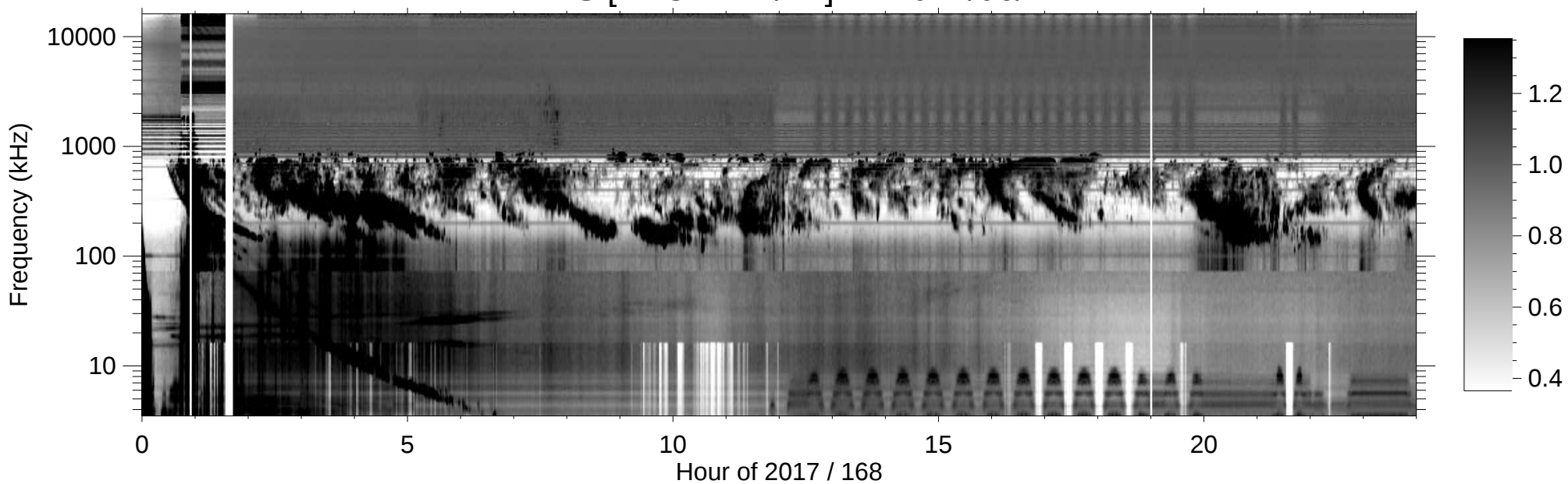
RPWS [ABCH1H2/Ex] (-B) 2017/06/17
