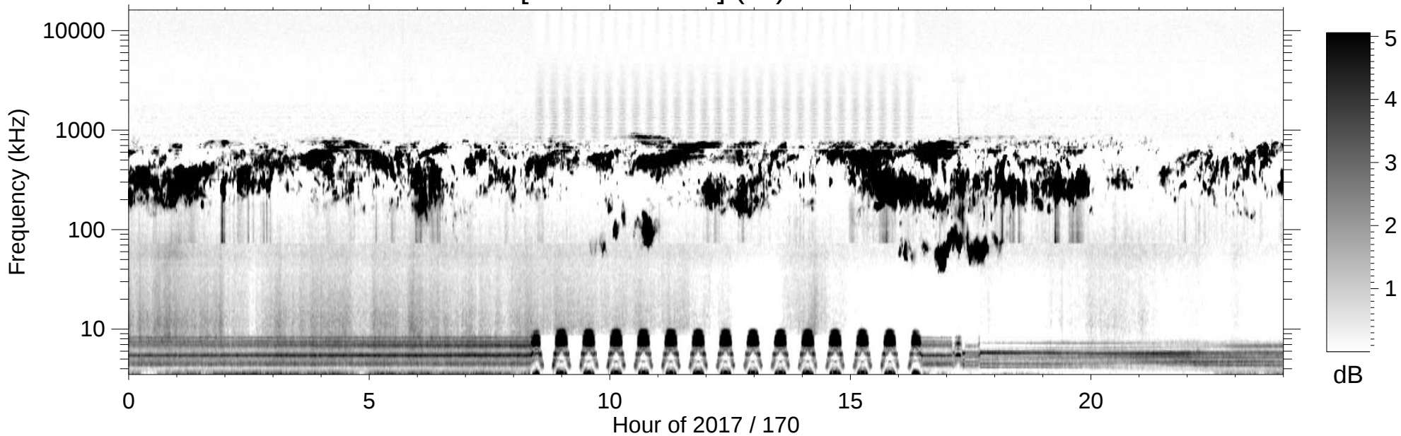
RPWS [ABCH1H2/Ex] (-B) 2017/06/19
