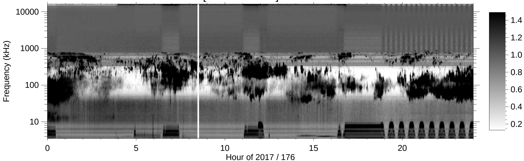
RPWS [ABCH1H2/Ex] (-B) 2017/06/25
