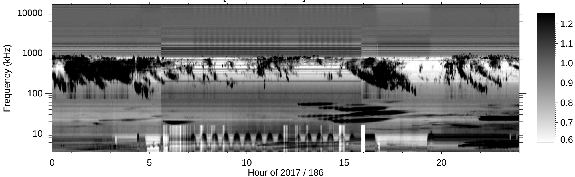
RPWS [ABCH1H2/Ex] (-B) 2017/07/05
